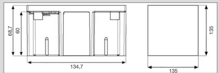
Paving Tray Box Installation Depth
