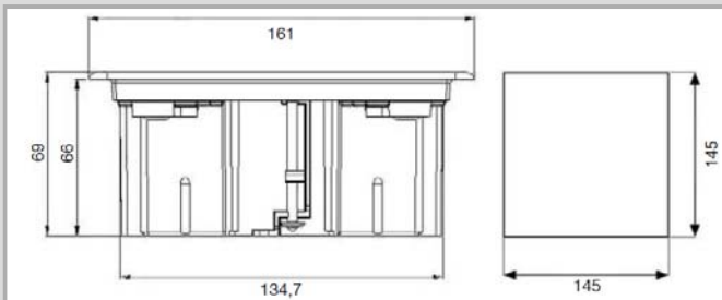
Raised Floor Tray Box Installation Depth
